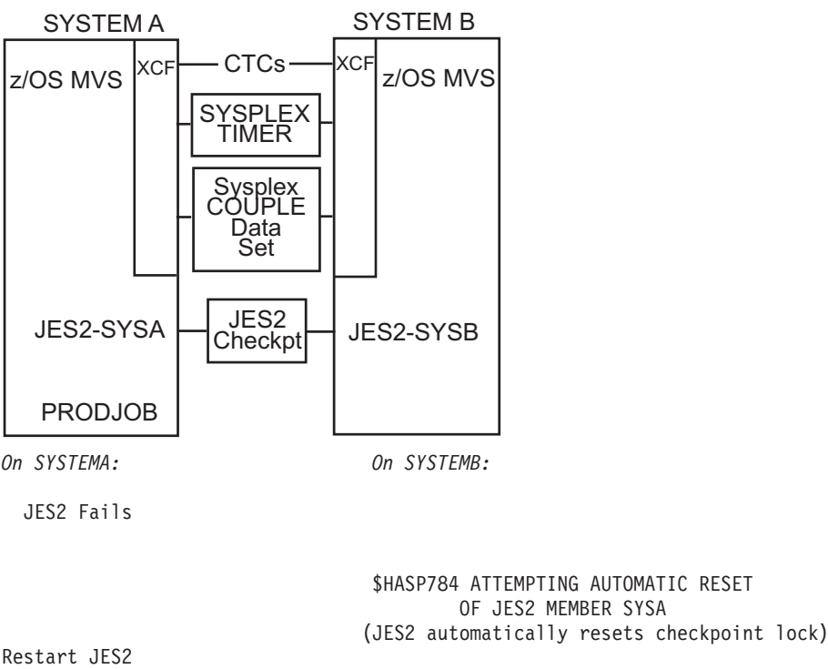
Figure 51. Sysplex with the AUTOEMEM Option Enabled, a JES2 Failure (Coupling Facility)
