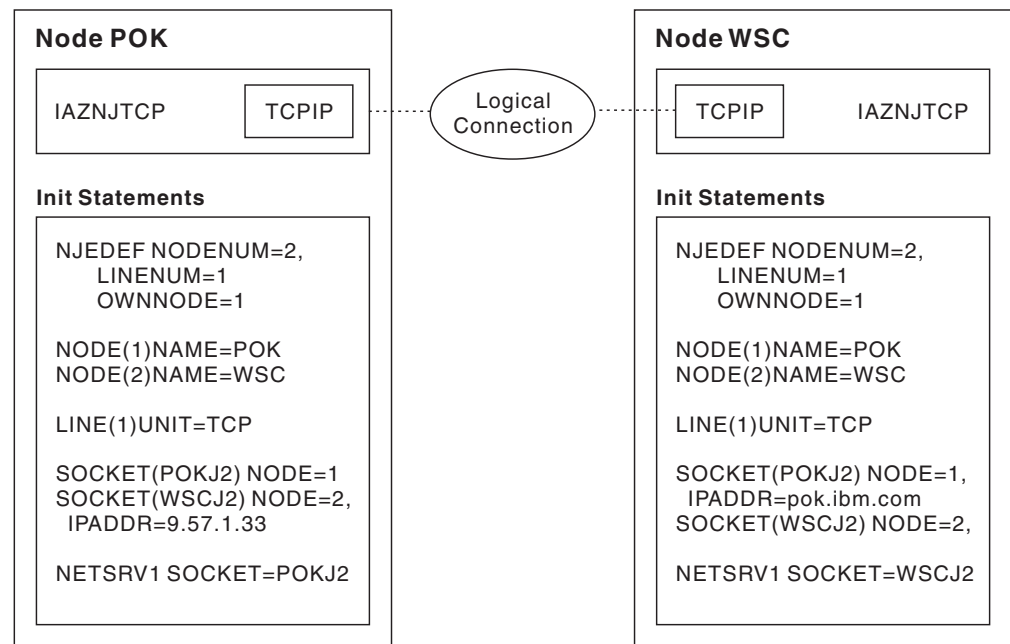
Figure 69. Example of a two node network and the JES2 initialization statements required to communicate between the two nodes using NJE/TCP
