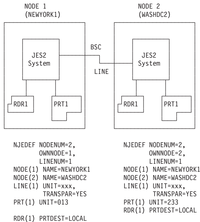
Figure 63. Minimum NJE Configuration (BSC only)
