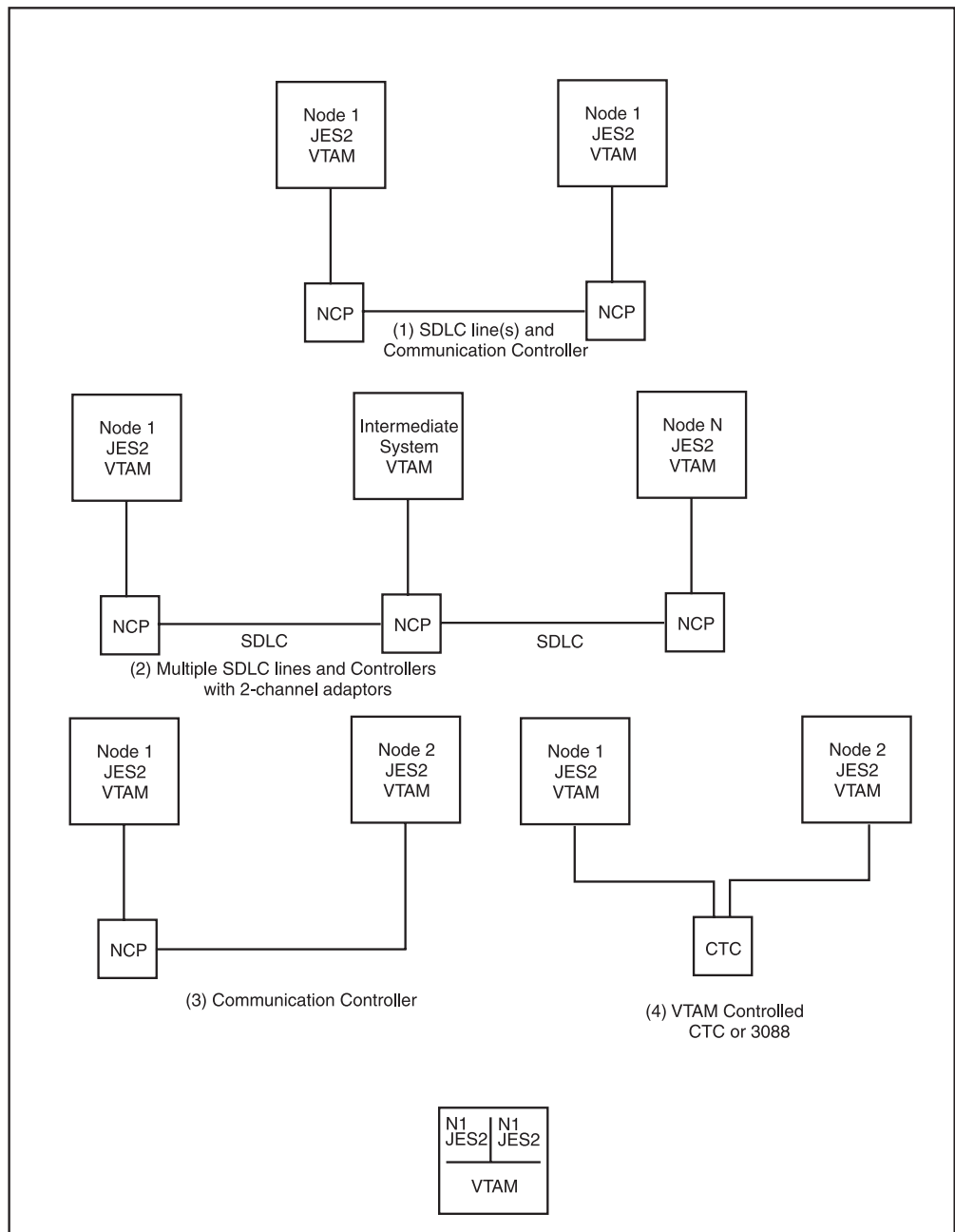
Figure 64. Basic SNA Configurations
