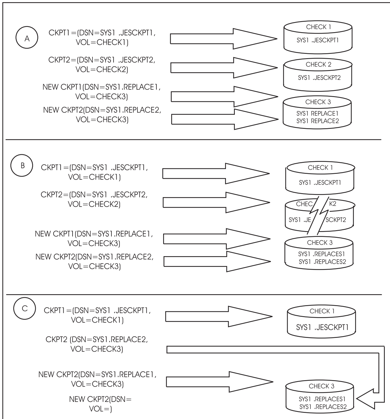
Figure 46. Example of Checkpoint Data Set Forwarding
