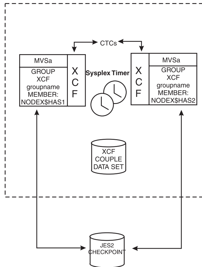
Figure 53. The JES2 AUTOEMEM Option in a Two-Member Sysplex Configuration
