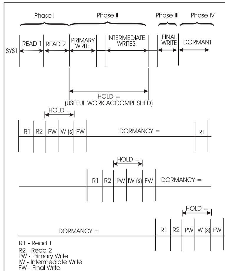
Figure 41. The Checkpoint Cycle (In a 3-Member Multi-Access Spool Environment)
