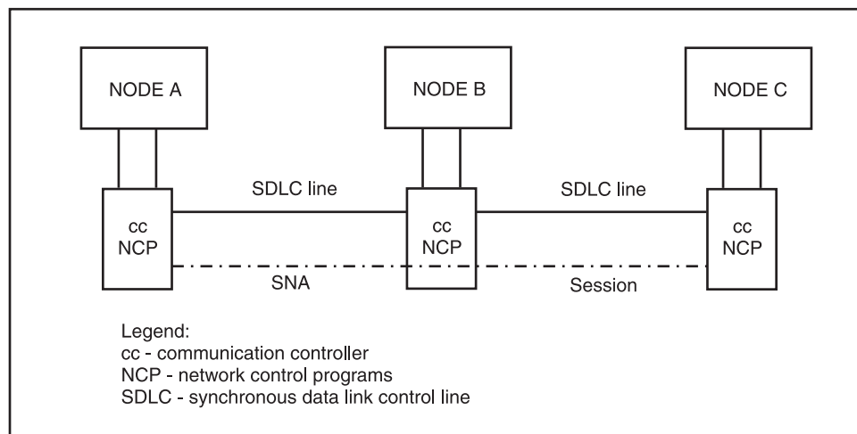
Figure 54. Simple SNA NJE Configuration
