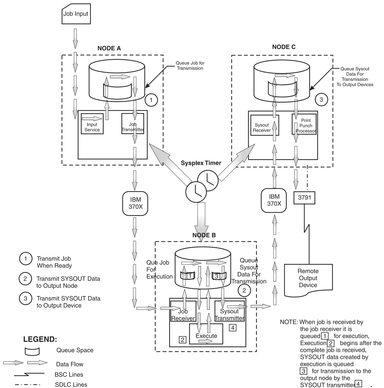
Figure 55. Processing Flow Through a Network
