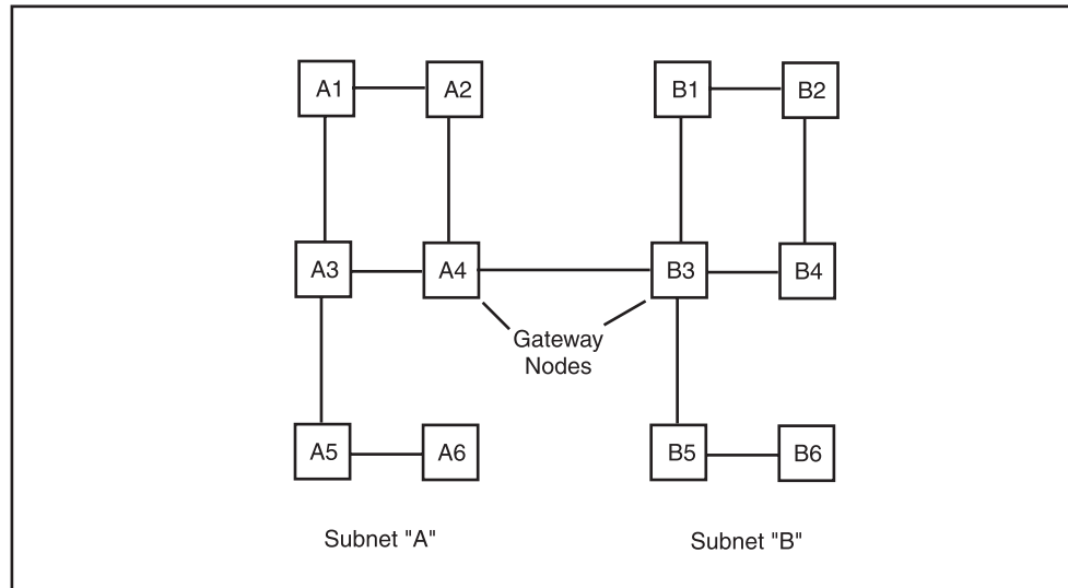
Figure 57. Gateway Configuration
