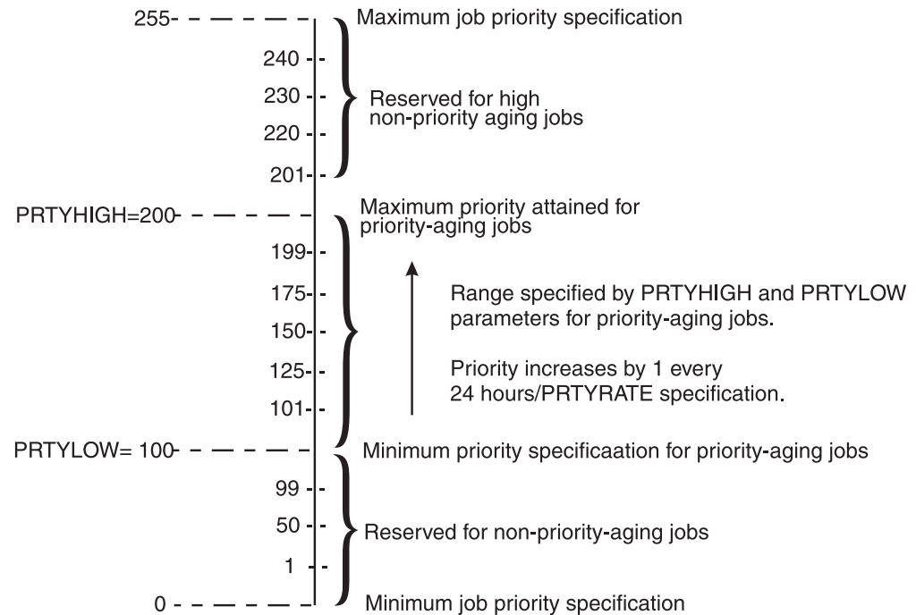
Figure 17. Example of the Interaction of Priority-Aging Parameters PRTYHIGH , PRTYLOW , and PRTYRATE on OUTDEF Statement
