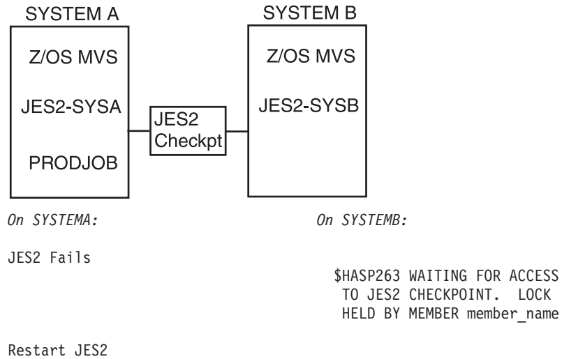
Figure 48. Two-Member MAS with JES2 Failure (Checkpoint on Coupling Facility)
