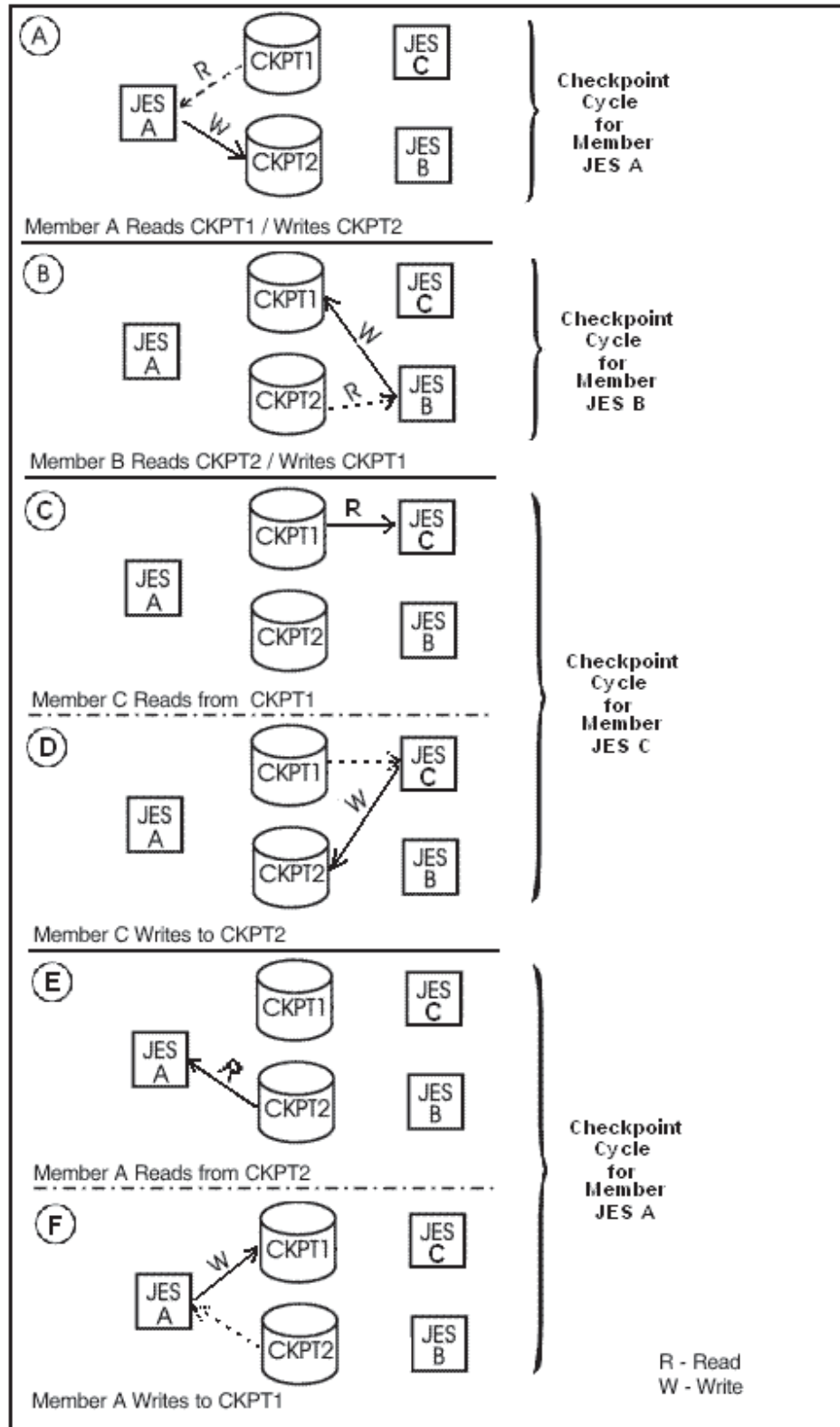
Figure 45. Checkpoint Data Set Processing -- DUAL Mode -- Three-Member Multi-Access Spool Configuration
