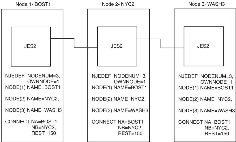
Figure 74. Static Connections
