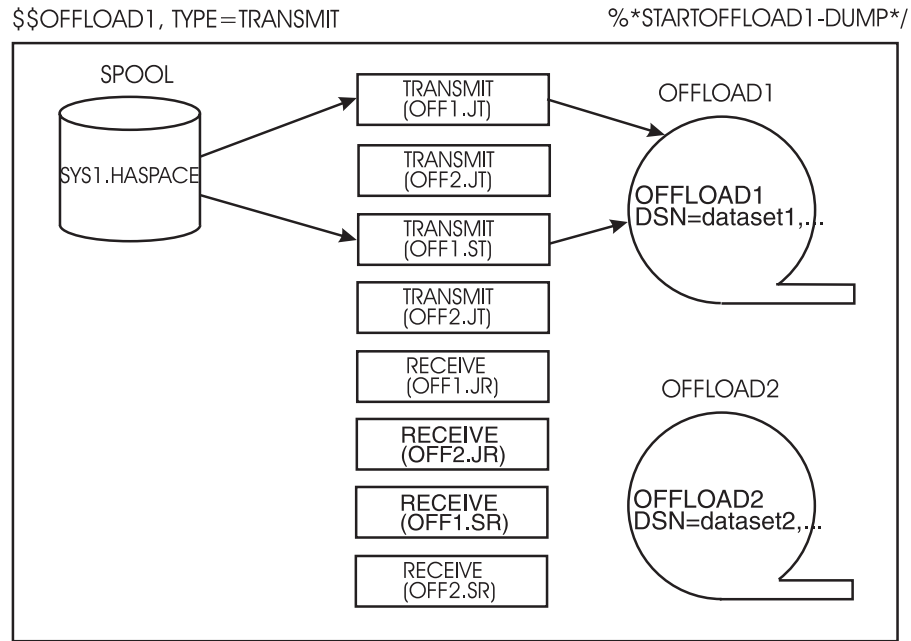
Figure 36. Offload Initialization Statements and $$ OFFLOADn,TYPE=TRANSMIT Relation
