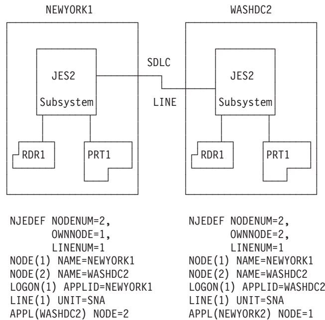
Figure 65. Minimum NJE Configuration (SNA)
