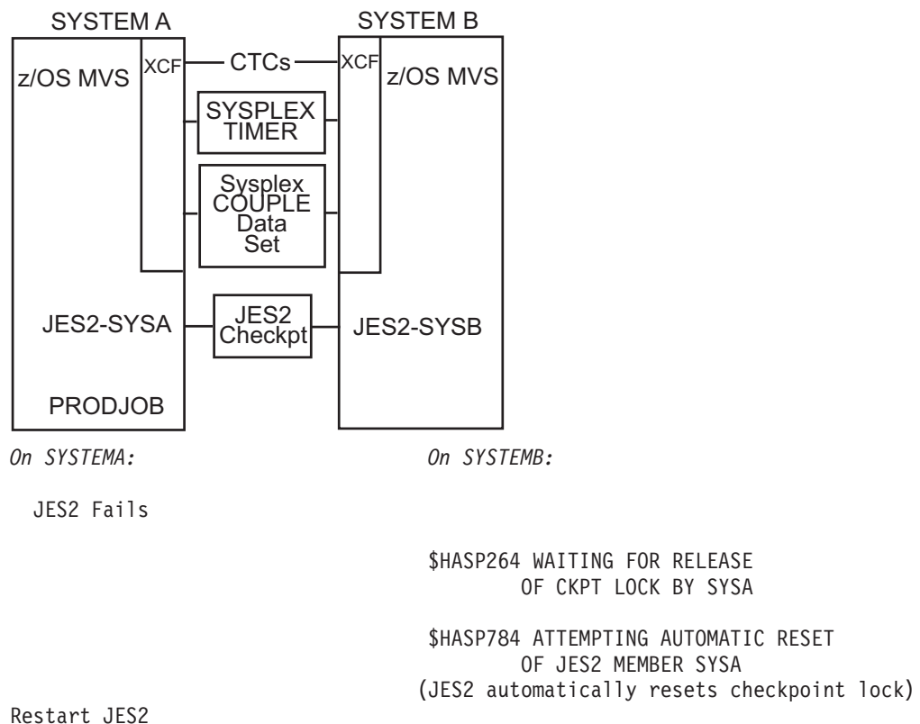
Figure 50. Sysplex with the AUTOEMEM Option Enabled, a JES2 Failure (DASD)
