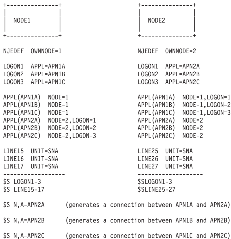
Figure 66. Parallel SNA NJE Sessions Between Two Nodes
